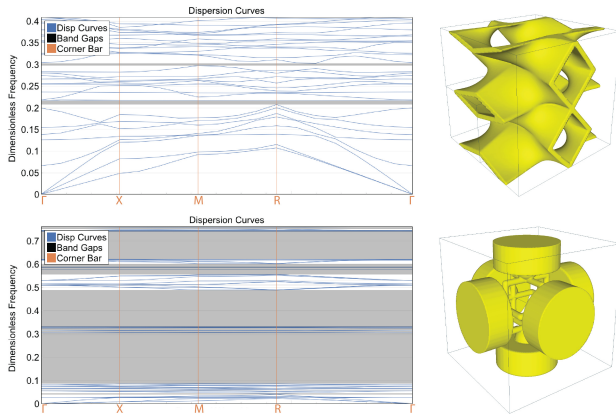
Fig. 12. Selected phononic bandgaps. We show the dispersion curves for two structures: (top) the randomly-generated shellular with the largest predicted bandgap and (bottom) the state-of-the-art metamaterial for phononic bandgap [Muhammad and Lim 2021]. Each dispersion curve plot shows normalized frequency values on the y -axis; the x -axis represents wave vectors along the irreducible first Brillouin zone for cubic-symmetric structures. Each vertical slice of the plot shows the structure’s eigenmodes under a particular wave vector; thus, any horizontal band without curves (gray) indicates a bandgap, i.e., a frequency range with no mode of transmission. Wide gaps in low frequency ranges are the most desirable.
