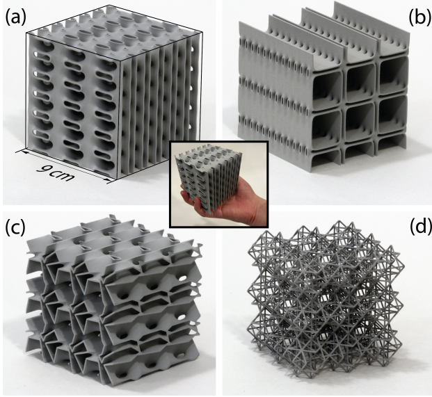
Fig. 10. Fabricated structures. We fabricated four structures based on our conjugate surface ((a) and (b)), direct surface (c), and truss-based (d) methods. We selected (a), (b), and (d) to maximize the ratio between Young’s modulus and density, subject to the constraints of the 3D printer ( \geq 1 mm thickness). Structure (c) is the result from Figure 11(c) (bottom). The middle photo shows the scale of our 3D-printed structures relative to the hand of an adult male.
