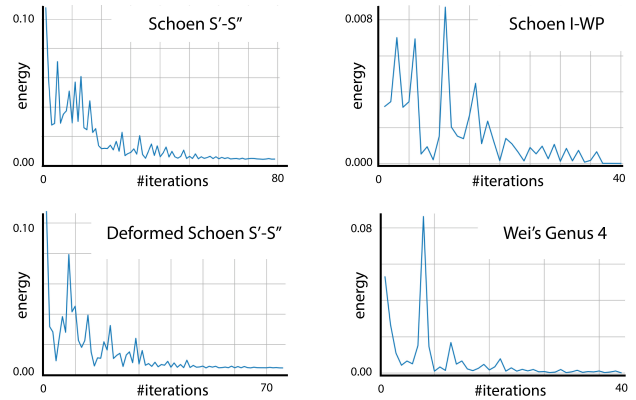
Fig. 7. Convergence of edge length optimization. We demonstrate convergence for the four TPMS with the longest optimization times, which use different FBVs: Schoen I-WP uses a prism, while the others use an AABBB.
