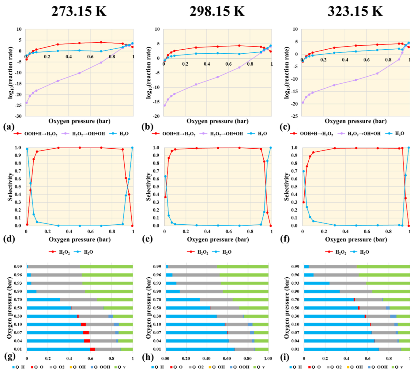
Figure 6. (a–c) Activity ( \text{OOH} hydrogenation, \text{H}_2\text{O}_2 decomposition, and \text{H}_2\text{O} formation), (d–f) selectivity ( \text{H}_2\text{O}_2 and \text{H}_2\text{O} ), and (g–i) proportion of main species coverage on Pd(100) as a function of oxygen partial pressure from 273.15 to 323.15 K ( P_{\text{O}_2} + P_{\text{H}_2} = 1 bar, P_{\text{H}_2\text{O}_2} = P_{\text{H}_2\text{O}} = 0.035 bar).
