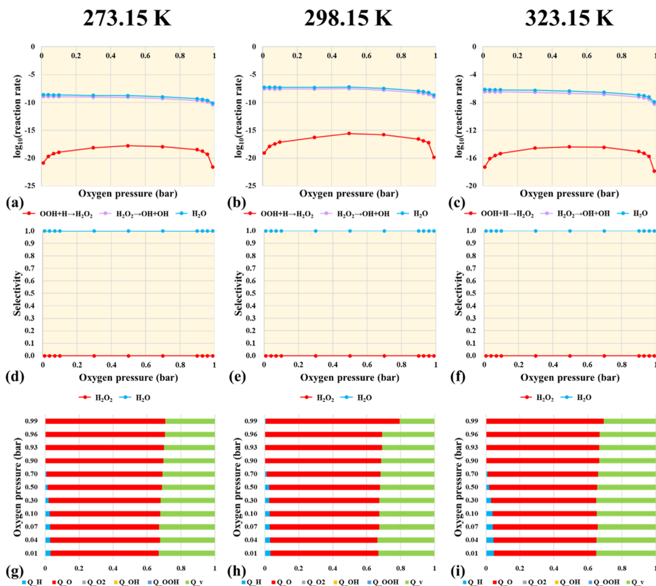
Figure 7. (a–c) Activity (OOH hydrogenation, H 2 O 2 decomposition, and H 2 O formation), (d–f) selectivity (H 2 O 2 and H 2 O), and (g–i) proportion of main species coverage on Pd(111) as a function of oxygen partial pressure from 273.15 to 323.15 K ( P_{O_2} + P_{H_2} = 1 bar, P_{H_2O_2} = P_{H_2O} = 0.035 bar).
