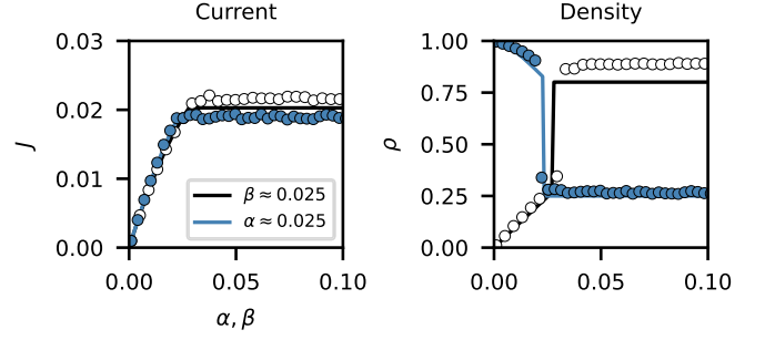
FIG. 13. Current and density as a function of entry and exit rates in an open-boundary TASEP with an infinite token pool. Left: Current at fixed \alpha = 0.025 (blue disks) as a function of \beta , or at fixed \beta = 0.025 as a function of \alpha (white disks) for k_+ = 0.1 and k_- = 0.02 . Current increases continuously with both parameters. Right: As in the left panel but for the density. While the current changes continuously, the density undergoes an abrupt change. These dependencies are correctly captured by the model (solid lines). Simulation data are from Fig. 12.
