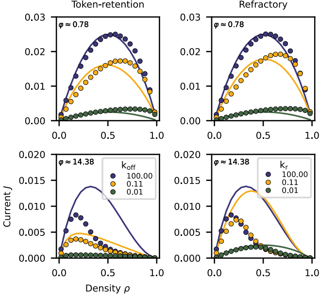
FIG. 20. Current as a function of density for the case of periodic lattice, finite tokens and two-stage progression of hopping particles. Figure shows current-density relations for a few representative values of token scarcity ( \phi , see the legend) for data shown in Fig. 4. Solid lines represent model predictions and markers denote simulation results.
