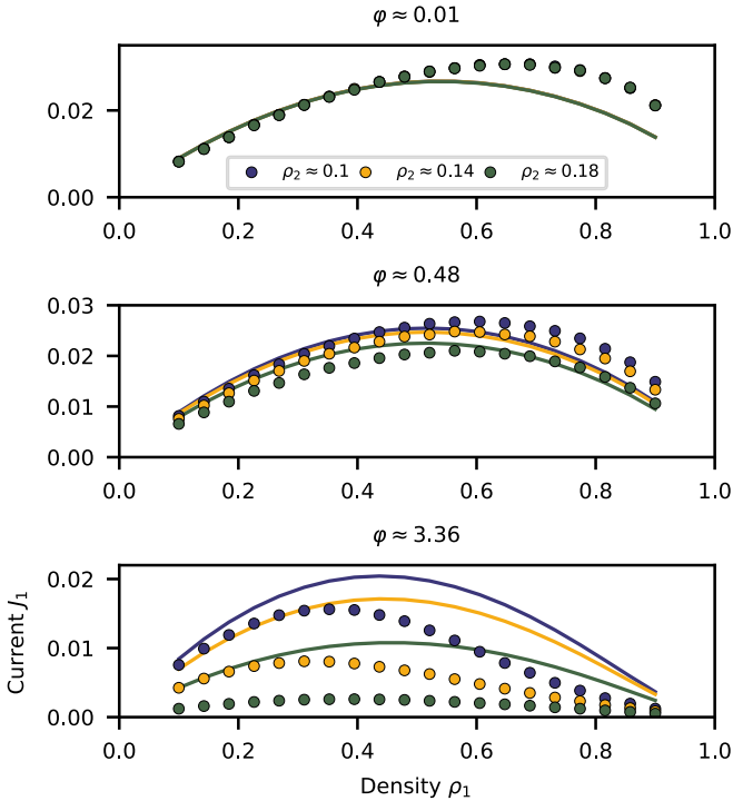
FIG. 21. Current as a function of density for the case of two competing periodic TASEPs with finite tokens. Figure shows current-density relations for a few representative values of token scarcity ( \phi , see titles) for data shown in Fig. 7 and for different particle densities of the competing TASEP. Solid lines represent model predictions and markers denote simulation results.
