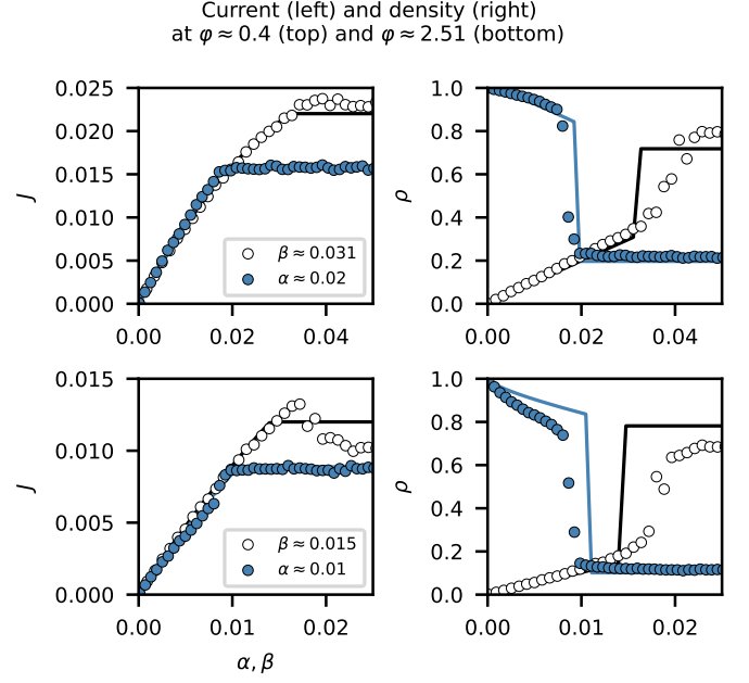
FIG. 22. Current and density as a function of \alpha, \beta as obtained in simulations and in modeling. Top: Simulation and model results for \phi \approx 0.4 . Left: Current at fixed \alpha (blue disks) or \beta (white disks); see legend for values of fixed quantities. Note a continuous increase in current with increasing \beta and \alpha , respectively. Solid lines correspond to model predictions. Right: As in the left panel but for the density. Bottom: As for the top panels but for \phi = 2.51 . Simulation data are from Fig. 14.
