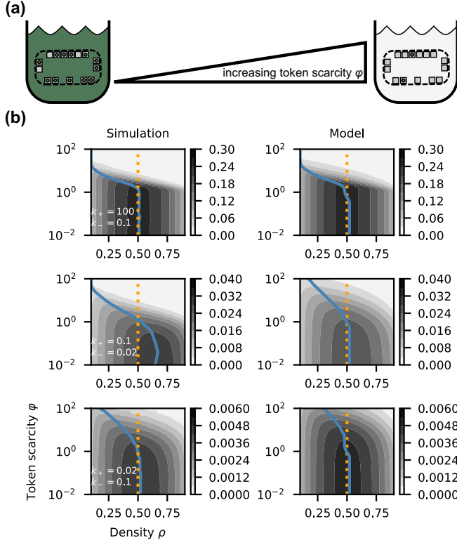
FIG. 3. Token scarcity influences the current-density relation. (a) Token scarcity \varphi quantifies total number of tokens relative to the number of lattice sites [Eq. (13)]. (b) Current-density relation surfaces for a finite token pool: simulation (left column) and analytical prediction (right column). Current is depicted in grayscale (bars at right). Shown are three examples with different binding parameters. Blue lines denote the point of maximal current at a given \rho ; smoothed by LOESS to mitigate parameter discretization grid. Orange dashed line denotes the position of current maximum for standard TASEP at \rho = 1/2 . Both model and simulation results were evaluated on a 20 \times 100 grid. Detailed cross sections of the surfaces are in Fig. 19.
