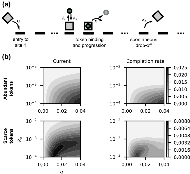
FIG. 15. Spontaneous particle dropoff in token-driven open TASEPs. (a) Schematic of a token-driven open-boundary TASEP with spontaneous particle dropoff. Particles without a token drop from the lattice with characteristic rate k_d . (b) Current and completion rate as a function of drop-off rate k_d and entry rate \alpha for abundant ( \varphi = 0.01 , top row) or scarce ( \varphi \approx 15.8 , bottom row) tokens. Simulation is for k_+ = 0.1 and k_- = 0.02 over 50 \times 50 grid. To avoid the congestion at the end of the lattice, we set \beta = 100 .
