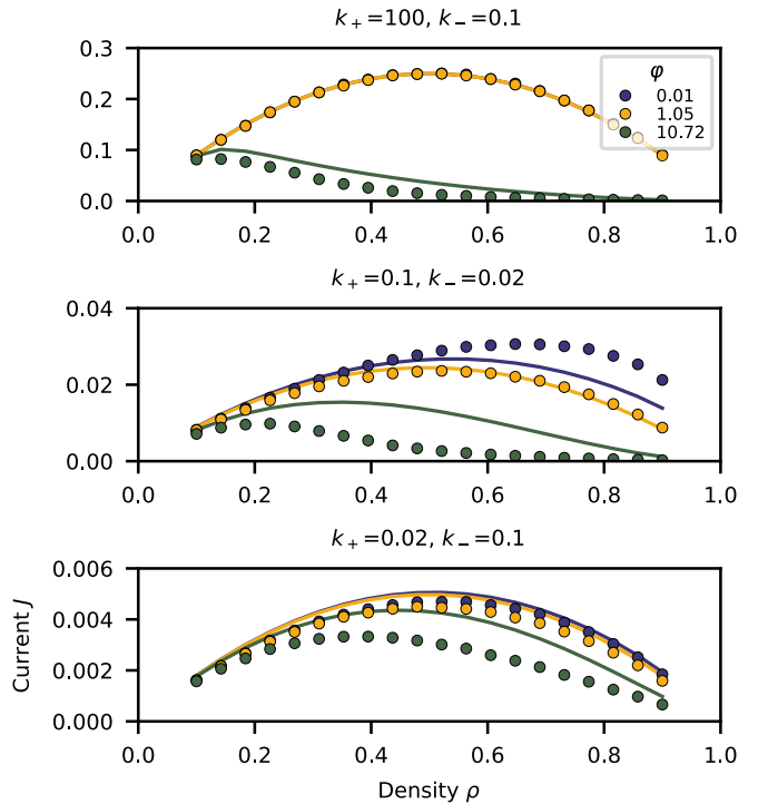
FIG. 19. Current as a function of density for the case of periodic lattice and finite tokens. Figure shows current-density relations for a few representative values of token scarcity ( \varphi , see legend) for data shown in Fig. 3. Solid lines represent model predictions and markers denote simulation results.
