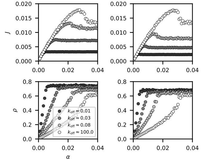
FIG. 23. Current and density as a function of \alpha obtained in simulations at \beta = 0.03 and \phi = 2.51 . Top: Current for particles with refractory (left) and token-retaining (right) state. Note that for k_r, k_{\text{off}} \gg k_+, k_-, p (white circles) we obtain the same bump in current relation. When k_r, k_{\text{off}} are reduced (see legend), the bump becomes slightly reduced at the expense of lower maximal current. Bottom: As on the top but for density.
