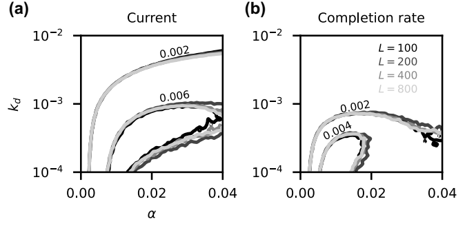
FIG. 18. Spontaneous particle dropoff in token-driven open TASEPs of different lengths. As Fig. 15, but for different lengths and only two contours are shown. For the shortest lattice ( L = 100 ), there are differences in the shape of the current and completion-rate surfaces when compared to longer lattices. As described in the main text, k_d was rescaled such that the drop-off rate \tilde{k}_d = k_d \times (200/L) remained constant for a given lattice length. Simulations are for k_+ = 0.1 and k_- = 0.02 , \varphi \approx 15.8 , and evaluated over 50 \times 50 grid. As is Fig. 15, we set \beta = 100 to avoid the congestion at the end of the lattice.
