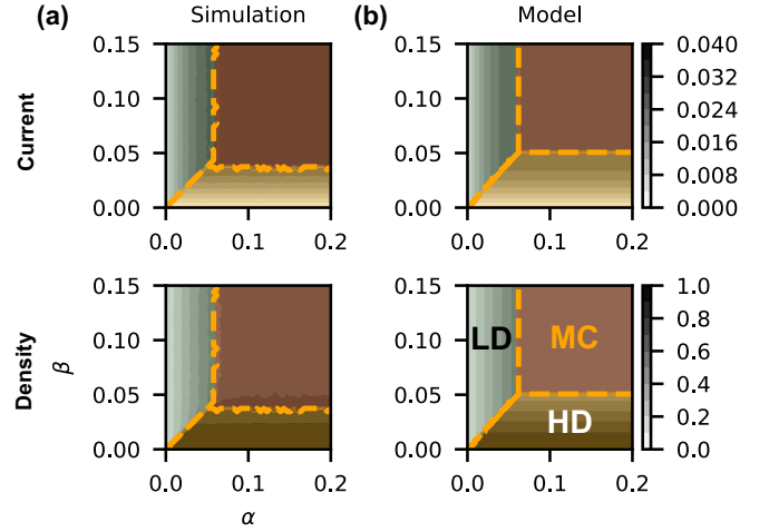
FIG. 12. Phase diagrams for open-boundary TASEP with an infinite token pool. (a) Simulation results obtained for k_+ = 0.1 and k_- = 0.02 over 50 \times 50 grid. Phase color code is as in Fig. 11. We estimated the phase boundaries between LD-HD and HD-MC phases by taking the first point at which density exceeds \rho_{\max} at a given \beta and first point at which current is equal to J_{\max} = J(\rho_{\max}) at fixed \alpha , respectively. (b) Same as for (a) but for model results.
