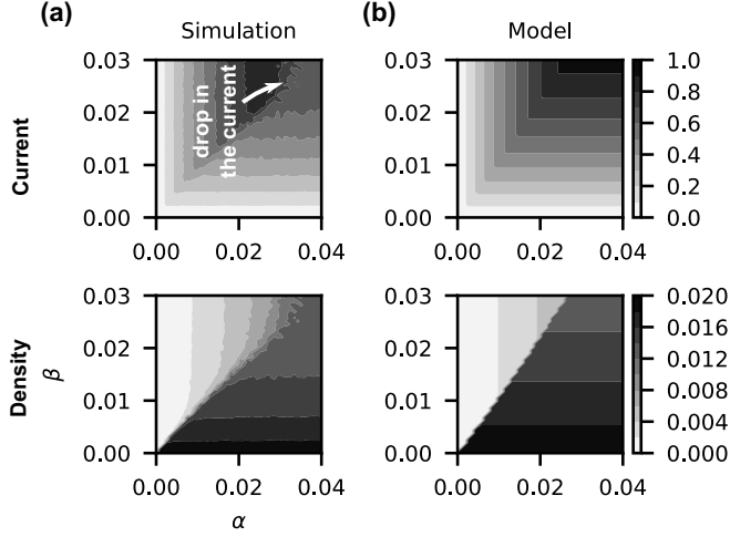
FIG. 14. Current and density for open-boundary TASEP with a finite token pool. Current (top row) and density (bottom row) are shown in gray scale as a function of entry and exist rates, \alpha and \beta . (a) Simulation and (b) model results, respectively, for \varphi \approx 2.51 . The model fails to predict the abrupt drop in the current (arrow) when \alpha passes a critical value for a given \beta . Results for k_+ = 0.1 and k_- = 0.02 , evaluated over 50 \times 50 grid.
