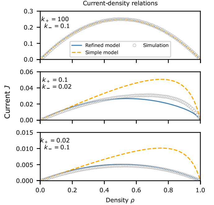
FIG. 2. Current-density relations for token-driven TASEP on a ring in an infinite token pool. Dependence of current on particle density changes with the kinetic rates k_+ and k_- . Rapid binding ( k_+ \gg p , k_- , top) results in the standard relation [Eq. (1)] between \rho and J that both the simple [Eq. (8)] and the refined [Eq. (10)] models predict correctly. Reducing k_+ , k_- lowers the maximal current and skews the relation towards higher \rho (middle), which is less pronounced if k_+ < k_- (bottom). Note: Simulation data completely cover the prediction of the refined model in the bottom panel and thus we made plot markers semitransparent.
