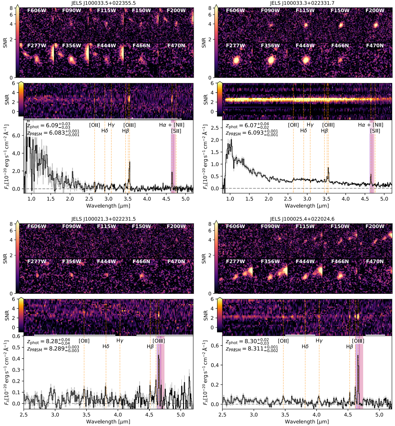
Figure 10. Example emission-line sources selected in JELS narrow-band imaging with spectroscopic confirmation from NIRSpec PRISM spectroscopy (DD 6585, PI Coulter). For each source, the upper panel shows photometry cut-outs (2 arcsec \times 2 arcsec) from HST/ACS (F606W) and JWST/NIRCam from both PRIMER and JELS. The lower panel for each source shows the corresponding standard pipeline reduced 2D and 1D PRISM spectra. A subset of bright rest-frame optical emission lines at the confirmed spectroscopic redshift are illustrated by the vertical dashed lines and corresponding labels. Shaded regions also show the wavelength coverage of the overlapping F466N and F470N filters for reference. The top row shows sources selected as H\alpha emitters, while the bottom row shows sources selected as robust z \sim 8.3 [O III] \lambda 5008 emitters. Note that at z \sim 8.3 , the width of the F466N/F470N narrow-bands is such that [O III] \lambda 4960 and [O III] \lambda 5008 (and potentially H\beta ) can be individually isolated from photometry alone.
