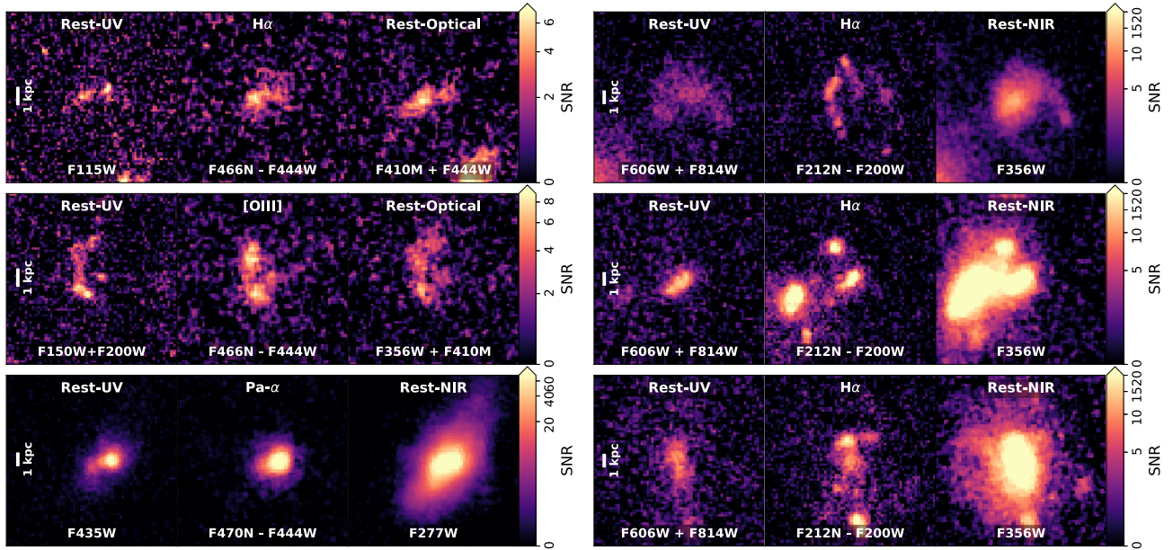
Figure 6. Illustration of resolved rest-UV (left), emission-line (centre) and rest-frame optical/NIR (right) for H\alpha , [O\text{ III}]\lambda 5008 and \text{Pa}\alpha emission-line objects in JELS. Examples of F466N or F470N-selected sources are shown in the left column, with examples of bright extended F212N excess sources shown in the right column. The corresponding broad and narrow-band filter combinations are indicated in each image. Cut-outs are 2\text{ arcsec} \times 2\text{ arcsec} in size, with consistent colour scales illustrated by the corresponding colour bar and 1 proper kiloparsec at the corresponding redshift shown for reference.
