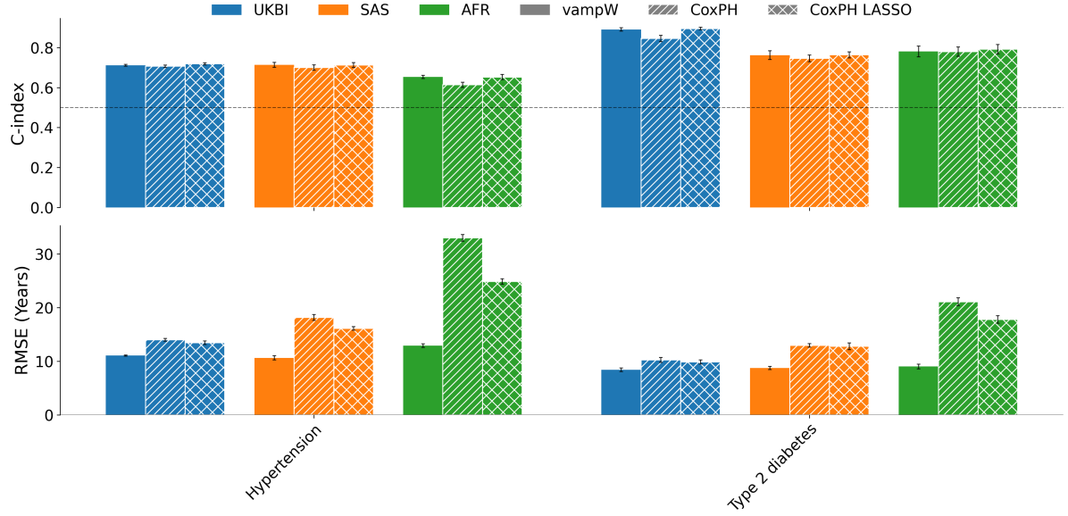
Figure C.12: Out-of-sample prediction performance across distinct genetic ancestries. We evaluate the predictive performance of vampW (solid bars), the standard CoxPH model (diagonal hatch lines), and CoxPH LASSO (cross hatch lines) across Hypertension and Type 2 diabetes traits from the UK Biobank. Results are stratified by genetic ancestry: British or Irish (UKBI, blue), South Asian (SAS, orange), and African (AFR, green). Performance is measured using the concordance index (C-index, top panel) and root mean squared error (RMSE in years, bottom panel). Phenotypic traits were included only if at least one minority ancestry group (SAS or AFR) contained a minimum of 200 total cases, ensuring that the 50% data splits retained at least 100 cases per split. The reported error bars represent the standard deviation across 10 splits, with each split evaluating a random 50% subsample of the dataset. We note that polygenic risk scores created by vampW are transferable to minority populations in the cohort; vampW exhibits similar C-index performance to Cox LASSO and outperforms the joint standard Cox model, while outperforming both competitor models in terms of the RMSE metric.
