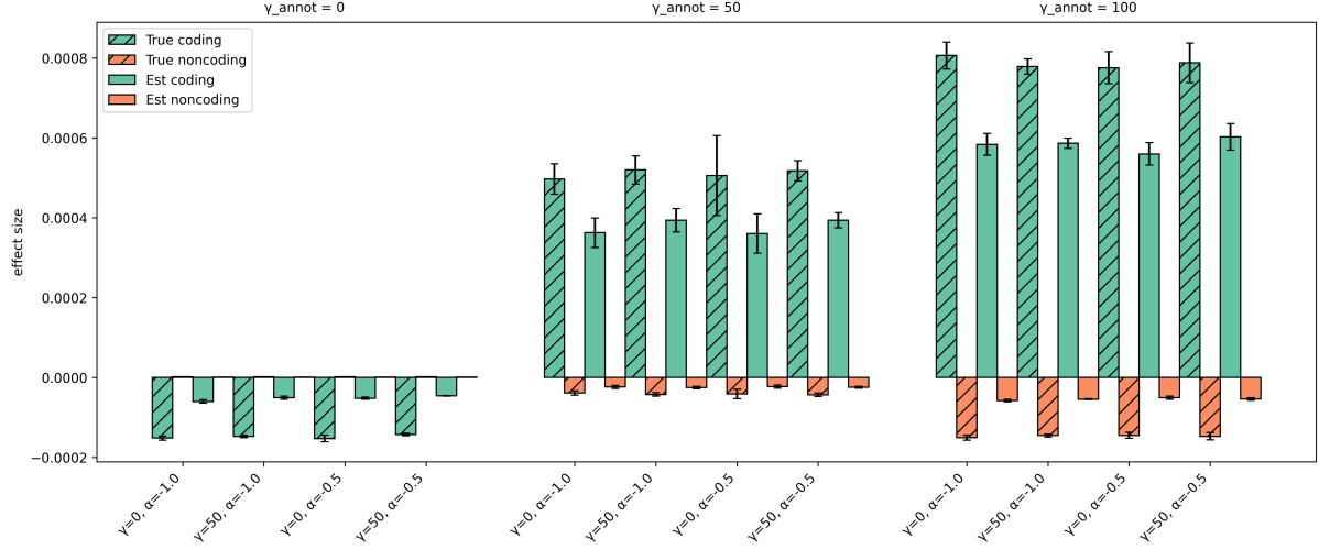
Figure B.7: Simulation study stratifying causal effects into coding and non-coding regions. We simulate 500 signals with a total heritability of h^2 = 7.25\% across a variety of settings for power law \alpha and percentage of common variants \gamma , also allocating \gamma_{\text{annot}} \in \{0, 50, 100\} % percentage of causal variants to the coding region of the DNA. Effect sizes ( y -axis) are calculated as the difference of the group average absolute value of the effects from the total group average absolute value of the effect (enrichment). The true simulated values are given by boxes with diagonal lines.
