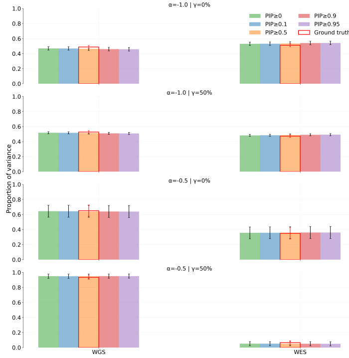
Figure B.6: Simulation study including WES burden scores alongside WGS variants from chromosomes 11 to 15 of the UK Biobank. We simulate 500 underlying causal signals with a total heritability of h^2 = 7.25\% , allocating 75% of signals to WGS variants and 25% to WES burden scores, with WES burden scores exhibiting effect sizes three-fold larger than those of individual WGS variants. For the detailed description of \alpha and \gamma parameters, see Methods. We find that the variance explained by WES and WGS, as inferred by gVAMP, aligns well with the ground truth across a range of PIP thresholds.
