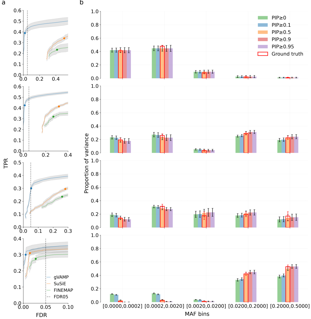
Figure 2.1: Simulation study of variable selection performance using whole genome sequence (WGS) data of chromosomes 11 to 15 in the UK Biobank. (a) Comparison of the true positive rate (TPR, y -axis) versus the false discovery rate (FDR, x -axis) between gVAMP (blue) and marginal GWAS association testing plus fine-mapping implemented in the FINEMAP (green) and SuSiE (orange) algorithms across four simulation scenarios. The rows of both (a) and (b) correspond to settings a , b , e , and f , which are described in the Methods, Supplementary Table B.1 and Figures B.1 to B.3, alongside additional simulation settings. For gVAMP, variable selection is conducted from posterior inclusion probability (PIP) values obtained from a single model run genome-wide. For FINEMAP and SuSiE, we use a Bonferroni corrected p -value significance threshold for marginal GWAS testing and then, having identified associated regions, we use the algorithms to obtain the PIP values to conduct variable selection. Error bands give the standard deviation across 5 simulation replicates. The blue, green and orange dots give the TPR and FDR at \text{PIP} \geq 0.95 threshold, which should correspond to an FDR of \leq 0.05 if the model correctly conducts variable selection based on PIP values. (b) The proportion of variance attributable to DNA loci of different frequency. We plot the proportion of the sum of the squared regression coefficients attributable to variants of different frequency as estimated from gVAMP across different posterior inclusion probability (PIP) thresholds. The ground truth (red frame) is calculated as the sum of squared true effects across different frequency groups. The variance attributable to SNPs of different frequency matches the ground truth when selecting variants at posterior inclusion probability \geq 0.5 . Error bars give the standard deviation across simulation replicates.
