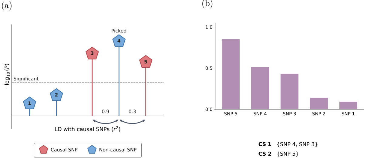
Figure 1.1: Conceptual overview of the fine-mapping process highlighting the limitations of marginal association testing influenced by LD structure. (a) Example of the correlation structure between causal and non-causal variants. The y -axis displays the significance of the marginal association testing. This example demonstrates that relying solely on a standard ranking of marginal associations fails to properly distinguish between causal and non-causal variants due to linkage disequilibrium. (b) The desired outcome of fine-mapping methods is the derivation of posterior inclusion probabilities for individual SNPs. These probabilities can then be used to construct credible sets (CS 1 and CS 2) with guaranteed false discovery control. This figure is adapted from [LZ25].
