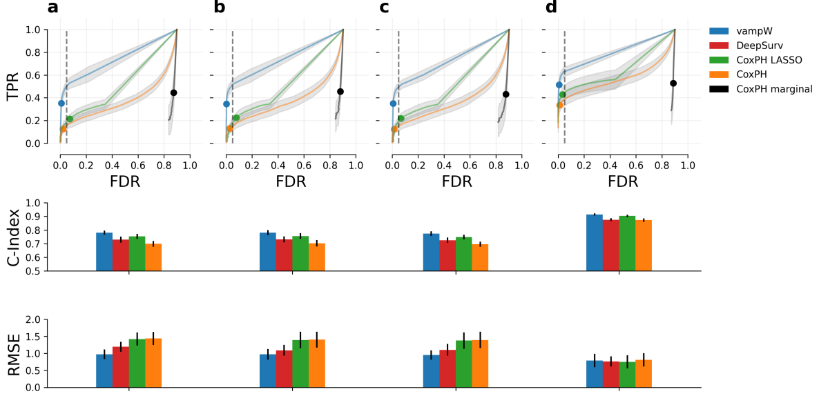
Figure 3.1: Simulation study of variable selection and out-of-sample prediction performance using 2,924 proteins across 53,018 individuals from the UK Biobank. We present four representative simulation scenarios (out of the 24 in total presented in Supplementary Figures C.1-C.3), covering low signal-to-noise ratios, model mis-specification, and high censoring rates. Specifically, subplots (a, b, c, d) correspond to simulation scenarios (m, o, q, t), as described in Supplementary Table C.1. Across all subplots, we use the following color convention: vampW in blue, marginal CoxPH in black, joint CoxPH in orange, LASSO-penalized CoxPH in green, and DeepSurv in red. In the first row, we show variable selection performance as the relationship between False Discovery Rate ( FDR = FP/(FP + TP) ) and true positive rate ( TPR = TP/(TP + FN) ). For vampW, we use posterior inclusion probabilities (PIPs), while for the other methods, p-value testing across multiple thresholds is employed, see Methods for details. Colored dots indicate the 0.95 threshold for vampW PIP and the Bonferroni-corrected 0.05 threshold for the other methods. The second row presents prediction performance measured by the concordance index (C-index) on a held-out test set. The last row presents prediction performance measured by the Root Mean Squared Error (RMSE) between the true and predicted survival times in the logarithmic domain, on uncensored individuals. The error bars (black lines in the bar plots and gray shaded areas in FDR-TPR plots) represent the standard deviation across 50 simulation replicates.
