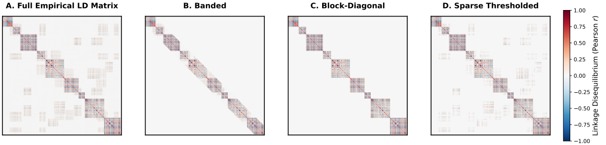
Figure 1.2: Visual comparison of common LD matrix approximations. This figure illustrates the structure of an LD matrix within a single chromosome, as interchromosomal LD is conventionally assumed to be negligible. (A) A full empirical LD matrix (Pearson correlation, r ), showing dense local block structures alongside diffuse polygenic background correlations and complex longer-range LD signals. (B) A banded approximation (e.g., utilized in LDpred models), where all correlations outside a strict bandwidth are set to zero. (C) A block-diagonal approximation (e.g., utilized in SBayesR), where the genome is partitioned into independent LD blocks and all off-block correlations are set to zero. (D) A sparse thresholded approximation, where all absolute correlations below a specified threshold are set to zero. While this approach preserves strong longer-range LD, it discards diffuse background correlations. Similar to the approximation errors introduced by matrix truncations, the zero inter-chromosomal LD assumption introduces further error. This assumption is the main difference between models operating on full individual-level data and those relying on LD matrices and marginal effect sizes.
