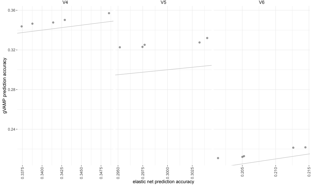
Figure B.17: Simulation study of out-of-sample prediction accuracy in UK Biobank imputed genotype data. We compare out-of-sample prediction accuracy ( y -axis) for polygenic risk scores (PRS) created at different sets of markers from gVAMP and an elastic net model implemented in the LDAK software. Grey lines give the 1:1 line. Comparisons are made across three settings: "V4" where 40,000 causal variants are randomly selected from 887,060 SNPs, with effects that contribute 50% to the phenotypic variance and have a power relationship to the minor allele frequency of -0.5, "V5" where 40,000 causal variants are randomly selected from 2,174,071 SNPs, with effects that contribute 50% to the phenotypic variance and have a power relationship to the minor allele frequency of -0.5, and "V6" where 5,000 causal variant effects are randomly selected from 2,174,071 SNPs, with effects that contribute 25% to the phenotypic variance and have a power relationship to the minor allele frequency of -0.5.
