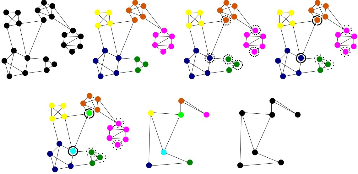
Figure 2.11: Main steps of the minimum cut algorithm. From left to right, top to bottom: Initial graph. Expander Decomposition. Run LocalKCuts from every vertex. Select only (1 - \epsilon) -boundary sparse cuts. Separate cuts from expanders to create clusters. Contract Clusters. Graph on which to recurse.
