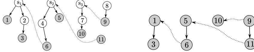
Figure 4.4: Illustration for the proof of Lemma 4.6.12, Case 1. Shaded nodes are informed nodes. Left: Solid lines represent E . Dotted lines are a suitable choice of a . Right: Solid lines represent F associated to E . Dotted lines represent b(a) . Any tree rooted at 9 on the right yields a suitable choice of a on the left.
