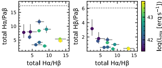
Figure 13. Paschen line ratios (left: H\alpha/Pa\beta and right: H\beta/Pa\beta ) versus Balmer decrement, colour-coded by L_{H\alpha} , for LRDs at z < 3.3 . Dotted lines indicate the expected value under the assumption of case B recombination. The very low H\beta/Pa\beta ratios support a scenario in which H\beta is resonantly scattered via H\alpha and Pa-\alpha .
