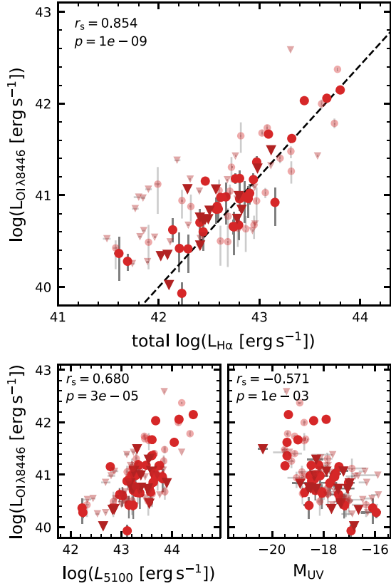
Figure 11. Correlation between the O I \lambda_{8446} line luminosity and the total H \alpha luminosity (top), and the continuum luminosity L_{5100} and M_{UV} (bottom). Large (small) symbols show the z < 4.5 (full) LRD sample, where triangles represent upper limits (95th percentile) in case of non-detections. The correlation with L_{H\alpha} is particularly strong; the best-fitting relation to the full sample (dashed line) is nearly linear, as the power-law slope \gamma = 1.17 \pm 0.07 .
