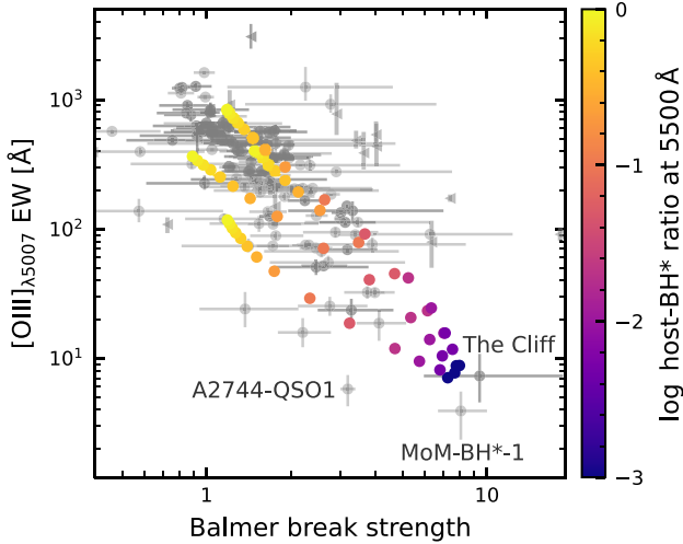
Figure 14. We investigate the strong correlation found between the [\text{O III}]_{\lambda 5007} EW and Balmer break strength (Fig. 10) empirically, by co-adding the spectra of The Cliff and low-mass ( M_* \sim 10^8 M_\odot ) star-forming galaxies for a wide range in host galaxy-to-BH* ratios and measuring the resulting [\text{O III}] EW and Balmer break strength. Our toy model, evaluated for four star-forming galaxy spectra, traces the slope and scatter of the observed distribution remarkably well. This suggests that LRDs can be described as the simple sum of a host galaxy and BH* component, and that variation in the host contribution alone can explain the weak [\text{O III}] lines observed in LRDs with strong Balmer breaks (L. J. Furtak et al. 2024; A. Graaff et al. 2025b; R. P. Naidu et al. 2026b).
