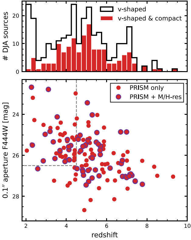
Figure 1. Top: redshift distribution of all PRISM spectra selected from the public DJA that satisfy the spectroscopic v-shape criteria of R. E. Hviding et al. (2025, black). The sample of v-shaped objects contains both LRDs and a large number of dust-reddened star-forming galaxies at cosmic noon. We define LRDs (146 unique sources; red) as the subset of sources satisfying strict compactness criteria in NIRCam/F444W imaging. Bottom: NIRCam/F444W magnitudes measured in circular apertures of radius 0.1 arcsec (half the MSA slit width) of all LRDs as a function of redshift. Of these sources, 40 per cent (58/146) also have medium- or high-resolution spectra from NIRSpc. Dashed lines indicate the subsample used for the modified blackbody fitting of Section 3.1.
