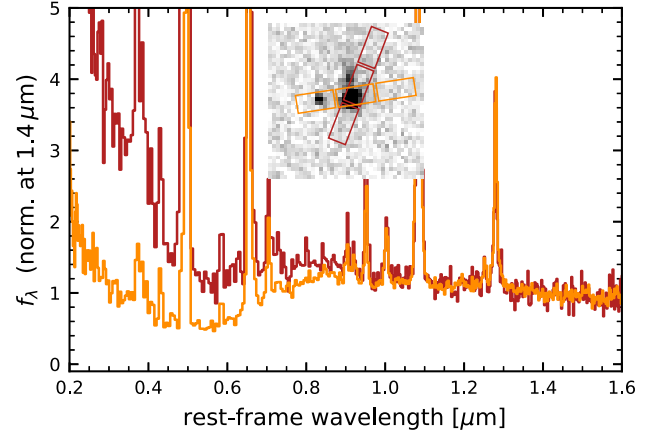
Figure A1. Duplicate spectra of NEXUS-10687 reveal that the precise slit placement can have a significant effect on the observed spectral shape due to the presence of extended blue emission in the northern vicinity of the LRD.
