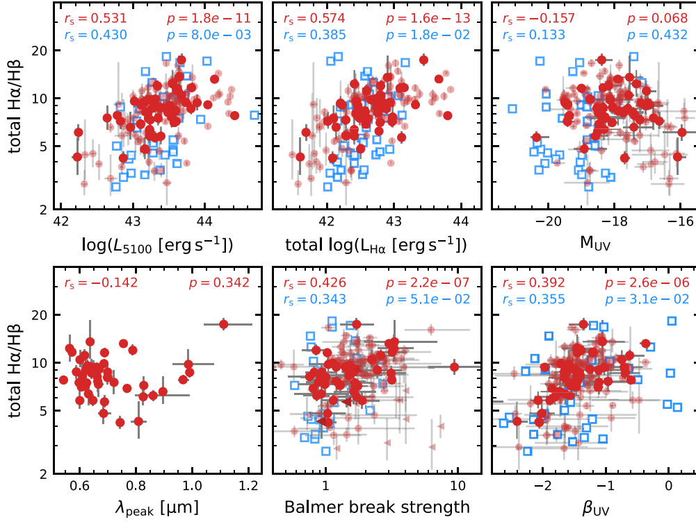
Figure 9. Balmer decrement of the total (broad+narrow) emission lines versus different luminosities (top) and spectral shape parameters (bottom). Symbols indicate the same as in Fig. 8. LRDs typically have high Balmer decrements ( H\alpha/H\beta \sim 10 ), which increase for sources with redder UV slopes. However, a lack of correlation with \lambda_{peak} argues against dust reddening as the cause. The Balmer decrement correlates strongly with both the rest-optical continuum and H\alpha luminosity, and weakly with Balmer break strength. This likely points to a luminosity-dependent population of hydrogen in the n = 2 state in the gaseous envelopes of LRDs, which in turns affects the balance between the collisional (de-)excitation and optical depths of the H\alpha and H\beta lines.
