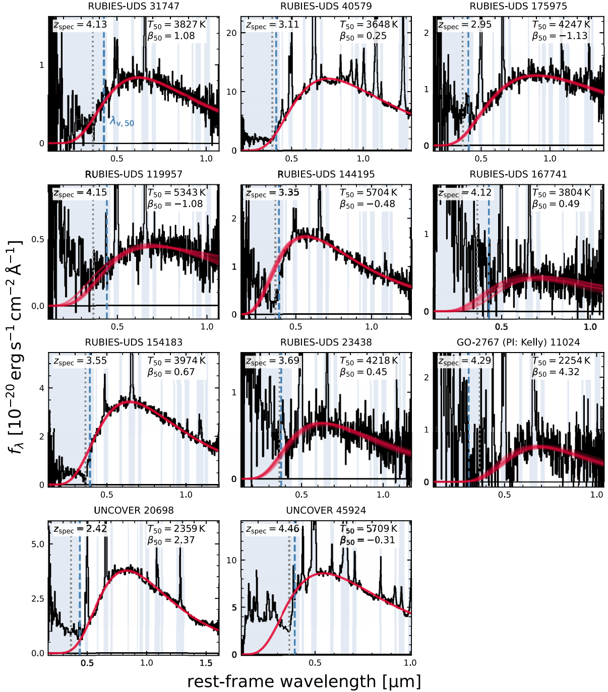
Figure C5. As Fig. C3, showing the third part of the z < 4.5 LRD sample.
