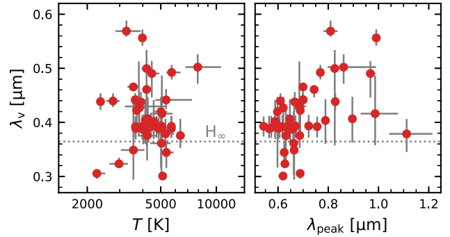
Figure 3. Location of the v-shape turnover wavelength \lambda_v versus modified blackbody temperature and \lambda_{\text{peak}} . For most LRDs, \lambda_v is near the Balmer limit (there is a small systematic bias, see the main text), but cooler LRDs with long peak wavelengths can have substantially larger \lambda_v than this.
