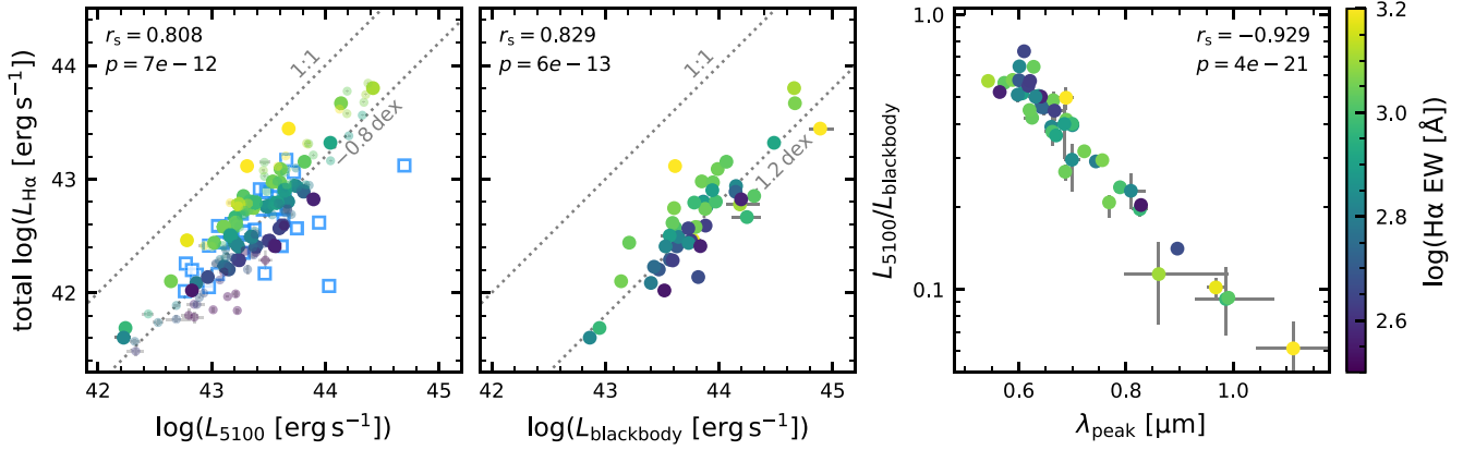
Figure 7. Total (broad + narrow) H\alpha line luminosity versus the luminosity at rest-frame 5100 Å (left) and integrated blackbody luminosity (middle), colour-coded by total H\alpha EW. Large (small) circles show the z < 4.5 (full) LRD sample, and blue squares the RUBIES broad-line sources of R. E. Hviding et al. (2025) that are not LRDs. Grey dotted lines indicate linear correlations, offset by a constant factor. The scatter about the unit slope is equally small (0.2 dex) for both L_{5100} and L_{\text{blackbody}} , despite the broad range in L_{5100}/L_{\text{blackbody}} spanned by the sample (right) as the two continuum luminosities are related via the peak wavelength. These tight relations point to a common origin for the production of the H\alpha lines and rest-optical continua of LRDs.
