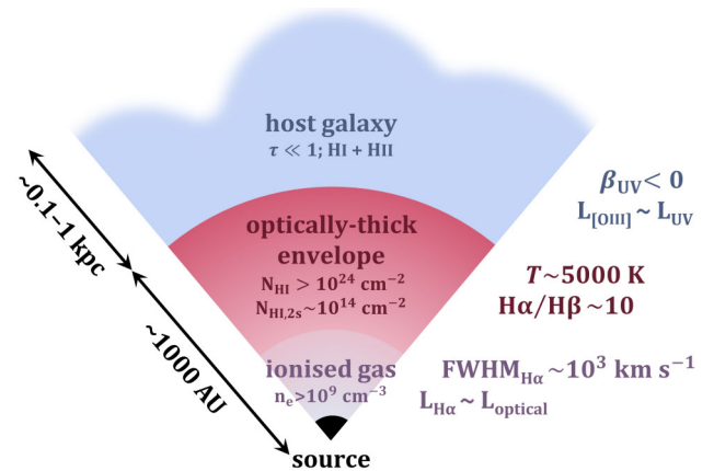
Figure 12. Schematic of the LRD’s gaseous structures discussed in Sections 5.1– 5.3.
