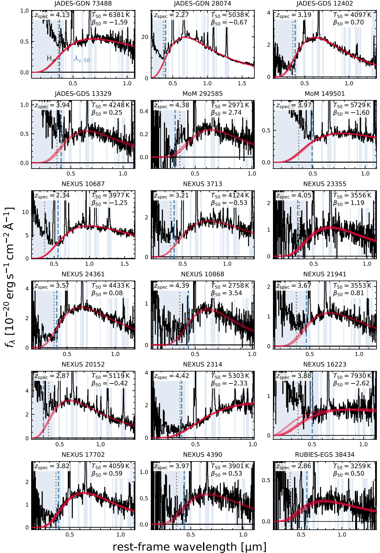
Figure C4. As Fig. C3, showing the second part of the z < 4.5 LRD sample.
