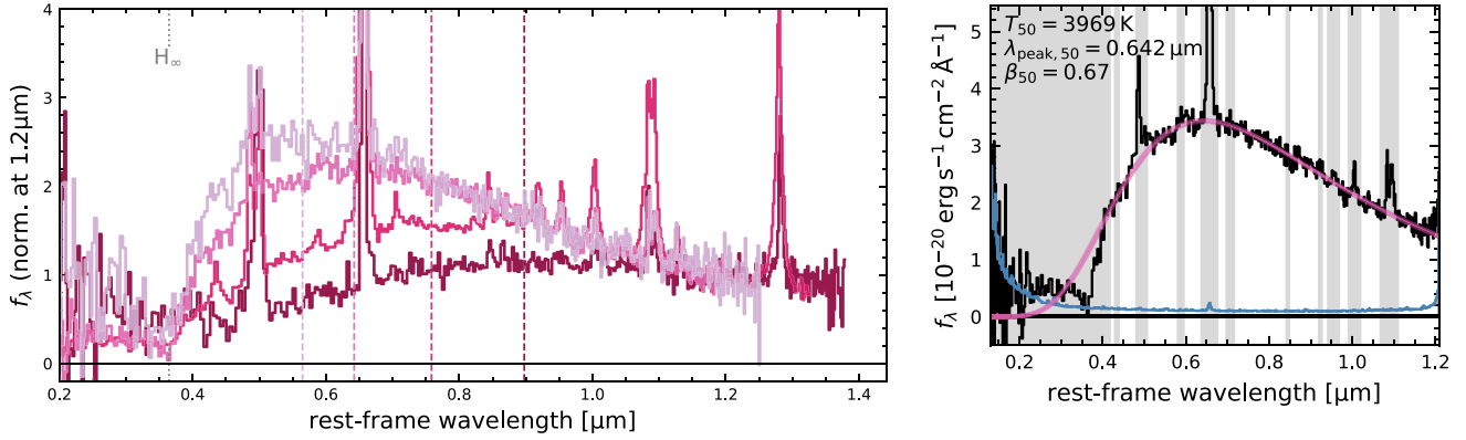
Figure 2. Left: NIRSpect/PRISM spectra (normalized at 1.2\,\mu\text{m} ) of four RUBIES LRDs showcasing their diverse spectral shapes. From light to dark: RUBIES-UDS-144195 (R. E. Hviding et al. 2025), The Cliff (A. Graaff et al. 2025b), RUBIES-BLAGN-1 (B. Wang et al. 2025), and RUBIES-UDS-175975. The colour-coded vertical dashed lines indicate the peak wavelengths of the modified blackbody fits to the spectra. Right: example of the three-parameter modified blackbody fitting to the PRISM spectrum of The Cliff , with its error spectrum shown in blue. Regions around strong emission lines and the region blueward of \lambda_v , marked in grey, were masked in the fit. Model lines (pink) represent 100 random draws from the parameter posteriors.
