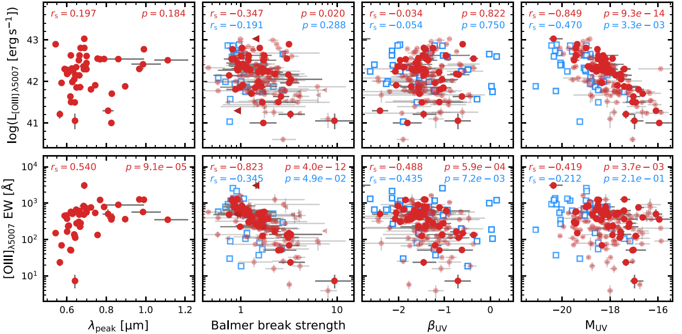
Figure 10. [O III] \lambda_{5007} line properties as a function of the optical continuum shape parameters ( \lambda_{peak} , Balmer break) and UV continuum properties ( \beta_{UV} , M_{UV} ). Symbols are as described in Fig. 8. The [O III] luminosity depends only on M_{UV} , but the EW is correlated strongly with the UV and optical SED shape, especially the Balmer break strength. For LRDs these trends are opposite to those found for H\alpha (Fig. 8), and indicate the [O III] emission has a different origin, likely from host galaxies.
