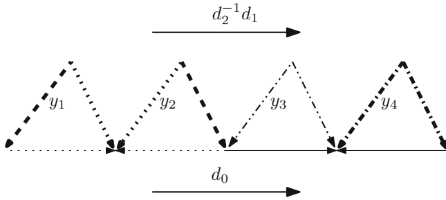
Fig. 3 Let g \in GF_1 with g = \overline{x_1 x_2 x_3 x_4} , where d_0(x_1) = d_0(x_2)^{-1} , d_0(x_3) = d_0(x_4)^{-1} , d_2(x_1) = d_1(x_2) , d_2(x_2) = d_1(x_1) , d_1(x_3) = d_2(x_3) and d_1(x_4) = d_2(x_4) . Simplicial set Y is then obtained by identifying faces of triangles y_1, y_2, y_3, y_4 as pictured here. One can see |Y| = S^2 \vee S^2
