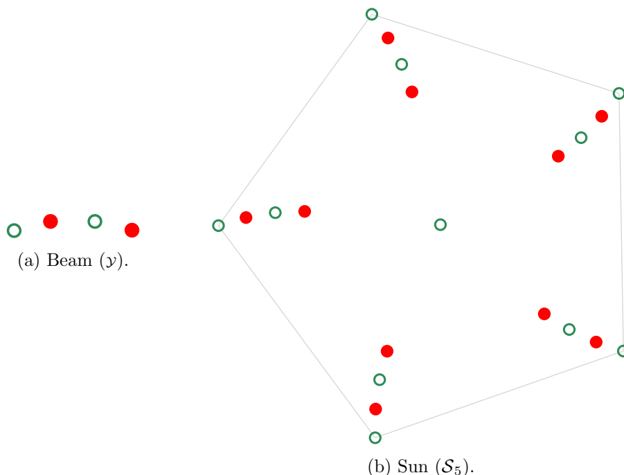
FIGURE 1. Sun configuration.
