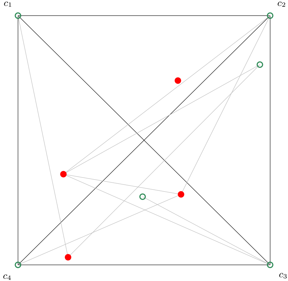
FIGURE 4. Counterexample to the No-reveal-move conjecture, with lines added for visual aid.
