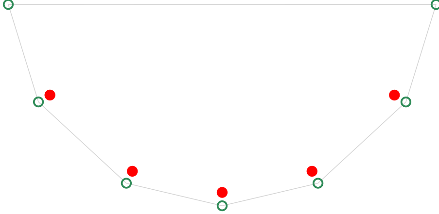
FIGURE 3. Moon ( \mathcal{L}_6 ).
